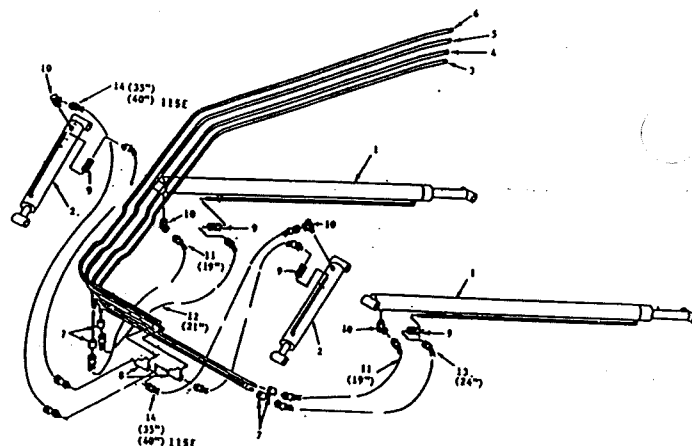
HYDRAULIC SYSTEM (for Models with Serial No. After 32695)
