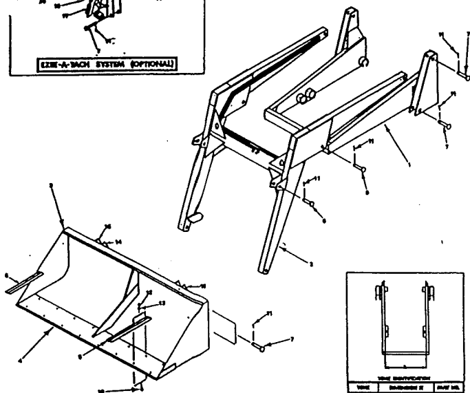
LOADER
