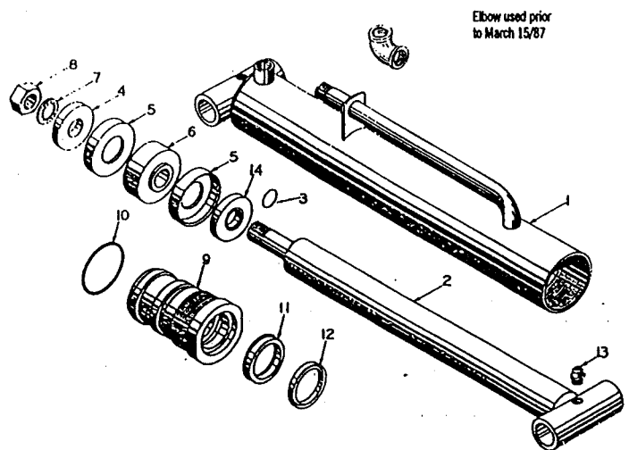
HYDRAULIC CYLINDER - H4 TYPE
