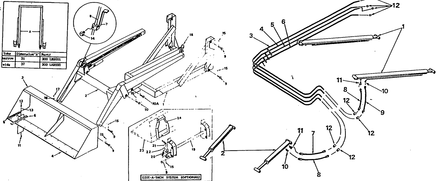
HYDRAULIC SYSTEM (for Models with Serial No. prior to 31642)
