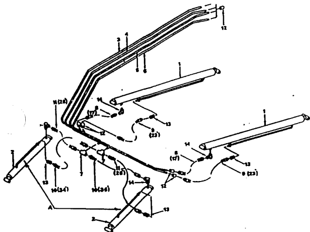
HYDRAULIC SYSTEM (for Models with Serial No. 32562 to 32952)
