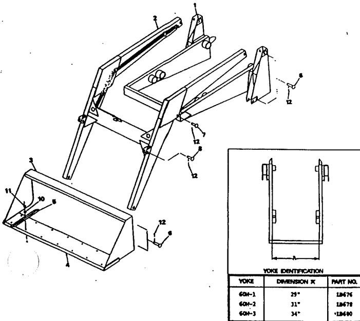
H-FRAME, YOKE & BUCKET
