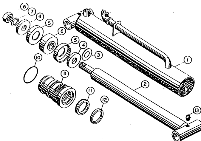
HYDRAULIC CYLINDER - N4 TYPE CYLINDER
