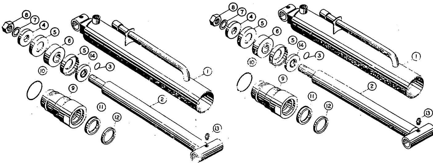
N5 THREADED HEAD TYPE BUCKET CYLINDER
