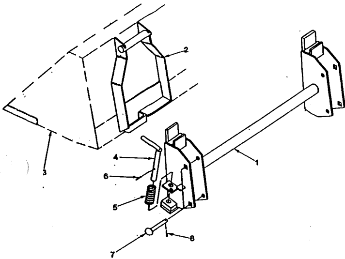
EZEE-A-TACH SYSTEM
