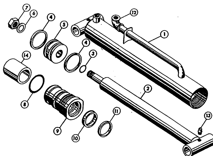
N4 THREADED HEAD TYPE CYLINDER DOUBLE "U" CUP PISTON
