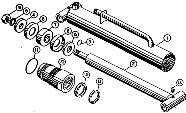
LIFT CYLINDER N4 THREADED HEAD TYPE A-CUP TYPE PISTON (for Models with Serial No. prior to 32182)
