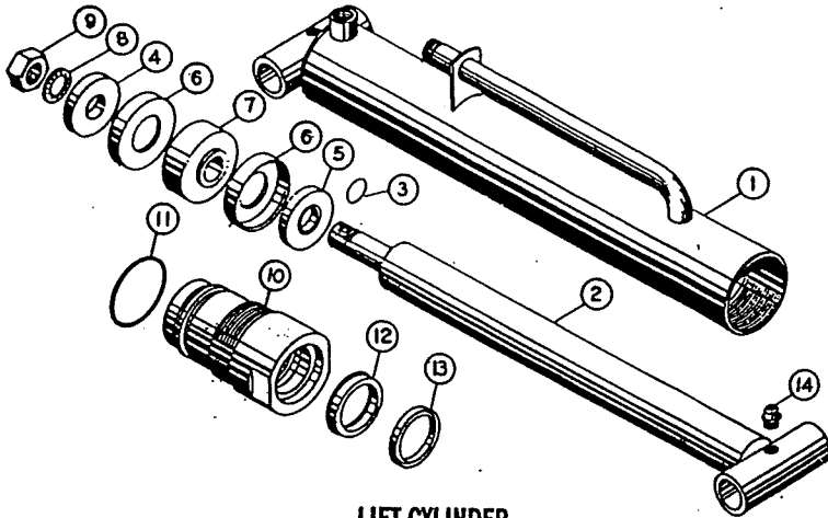
LIFT CYLINDER N4 THREADED HEAD TYPE A - CUP PISTON
