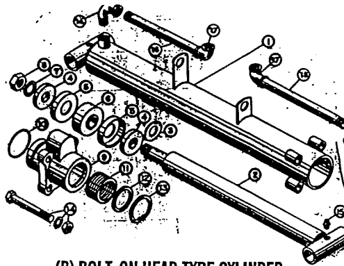
(B) BOLT-ON HEAD TYPE CYLINDER CODE NO. 39
