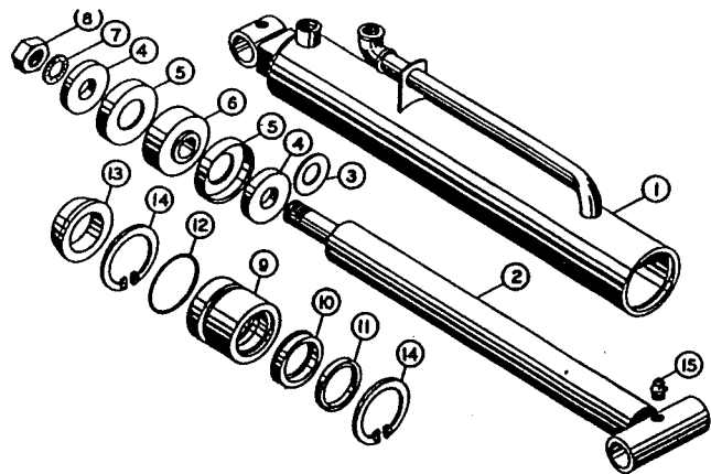
HYDRAULIC CYLINDER - S2 SNAP RING TYPE
