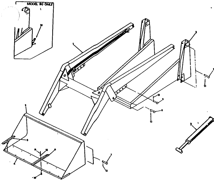
H-FRAME, YOKE AND BUCKET
