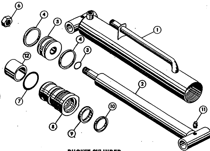
BUCKET CYLINDER N4 THREADED HEAD TYPE DOUBLE "U" CUP PISTON - Less Wear Ring
