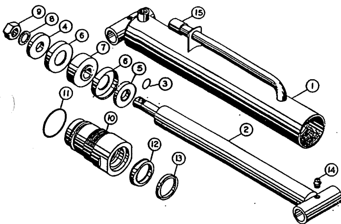
LIFT CYLINDER - N4 THREADED HEAD TYPE
