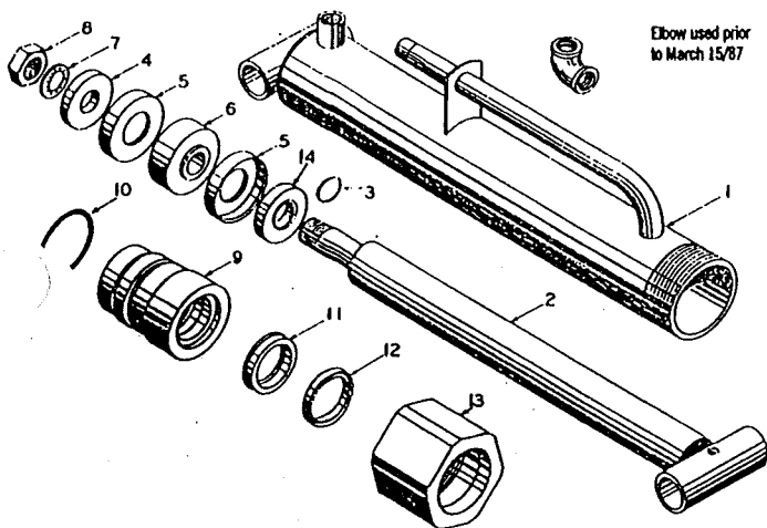
HYDRAULIC CYLINDER - H3 TYPE
