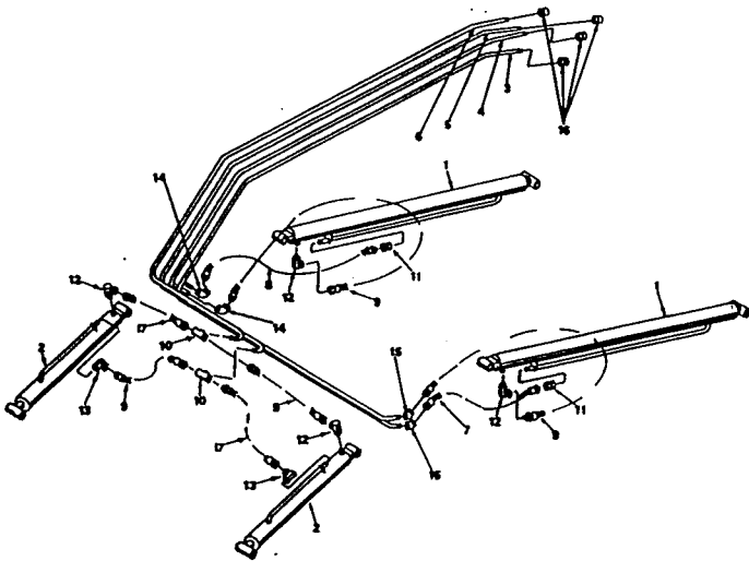
HYDRAULIC SYSTEM (FOR 60W LOADERS WITH SERIAL NO. 31398 TO 32150)
