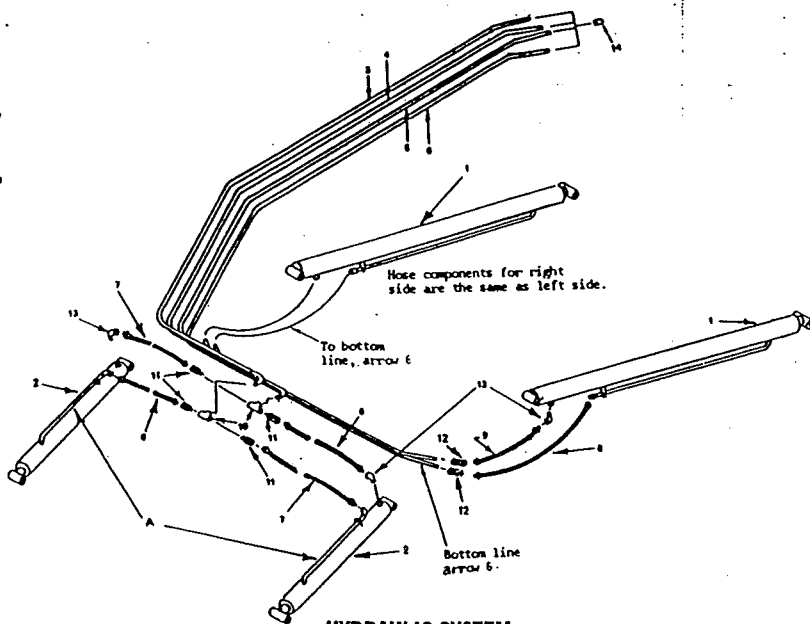
HYDRAULIC SYSTEM (for Models prior to Serial No. 31641)
