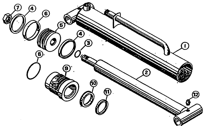
LIFT CYLINDER - N6 THREADED HEAD TYPE - U-CUP PISTON
