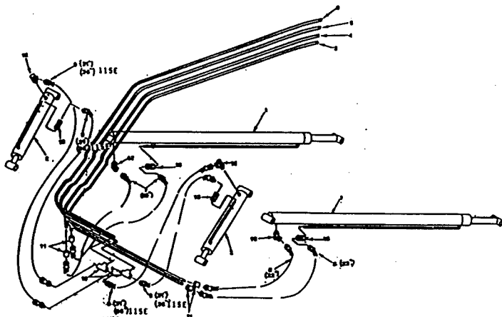
HYDRAULIC SYSTEM (for Models with Serial No. between 31583 and 32695)
