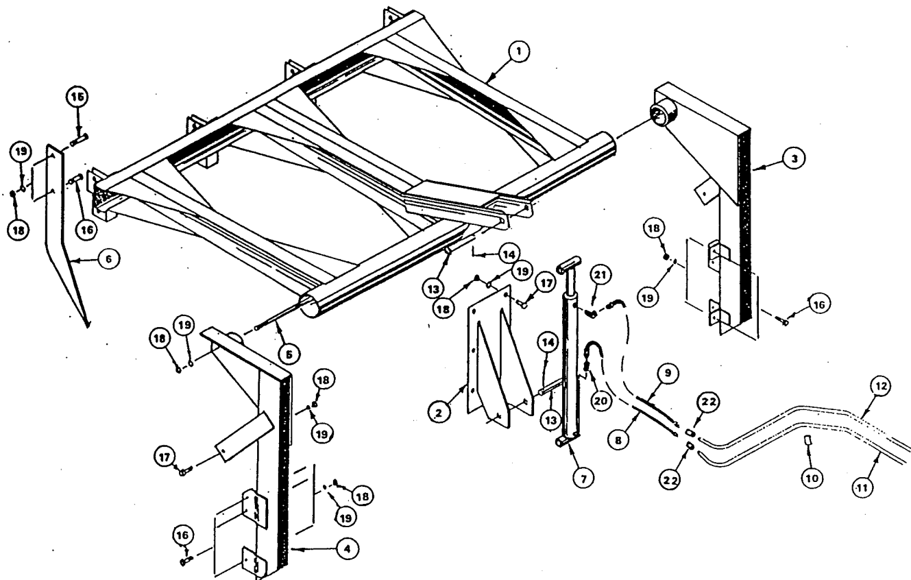
GRAPPLE FORK ATTACHMENT (FOR MODELS EQUIPPED WITH HYDRAULIC CYLINDER #243)
