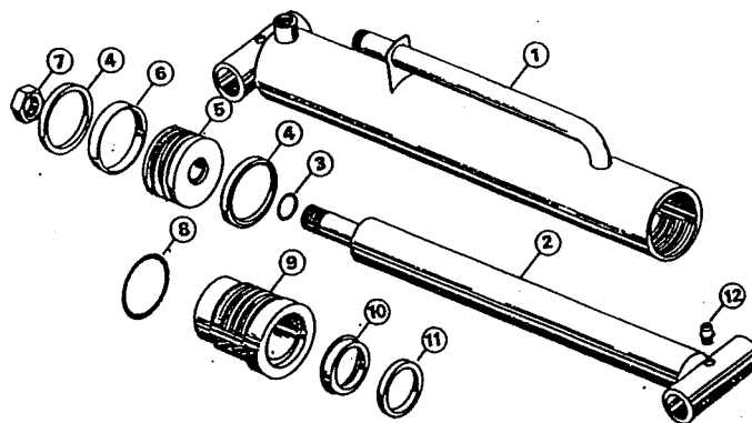
LIFT CYLINDER N4 THREADED HEAD TYPE DOUBLE U-CUP TYPE PISTON w/Wear Ring
