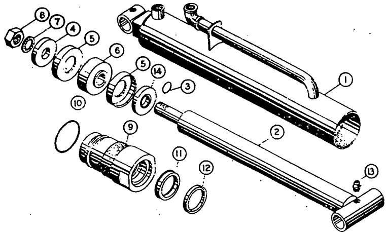
MODEL 30 & 40 BUCKET CYLINDER N5 THREADED HEAD TYPE
