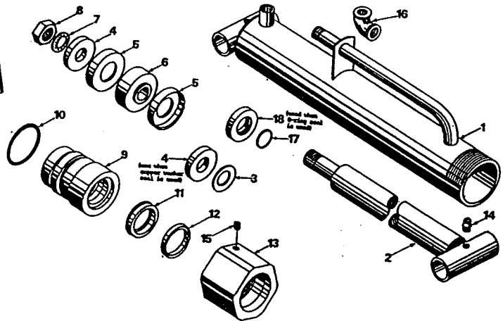
LIFT CYLINDER N3 EXTERNAL NUT TYPE
