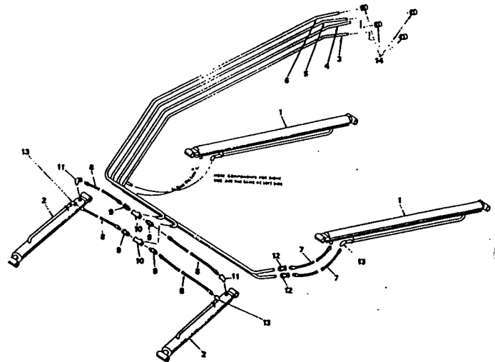
HYDRAULIC SYSTEM (FOR 60W LOADERS WITH SERIAL NO. PRIOR TO 31398)
