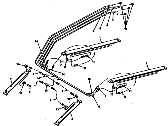
HYDRAULIC SYSTEM (FOR 60W LOADERS WITH SERIAL NO. 32150 AND UP)
