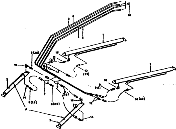
HYDRAULIC SYSTEM (for Models with Serial No. 31641 to 32094) * with the exception of 31652 and 31662
