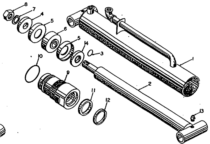
HYDRAULIC SYSTEM - N5 CYLINDER
