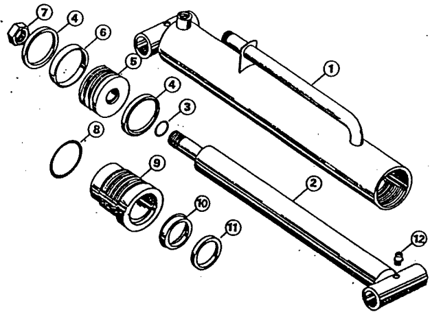
LIFT CYLINDER N4 THREADED HEAD TYPE DOUBLE U-CUP TYPE PISTON w/Wear Ring
