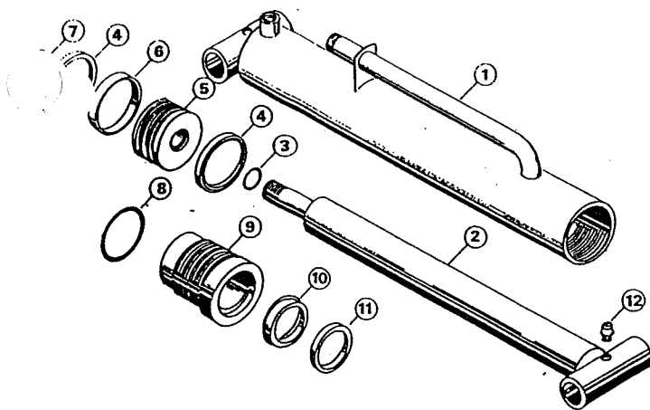
HYDRAULIC CYLINDER N4 TYPE DOUBLE "U" CUP PISTON
