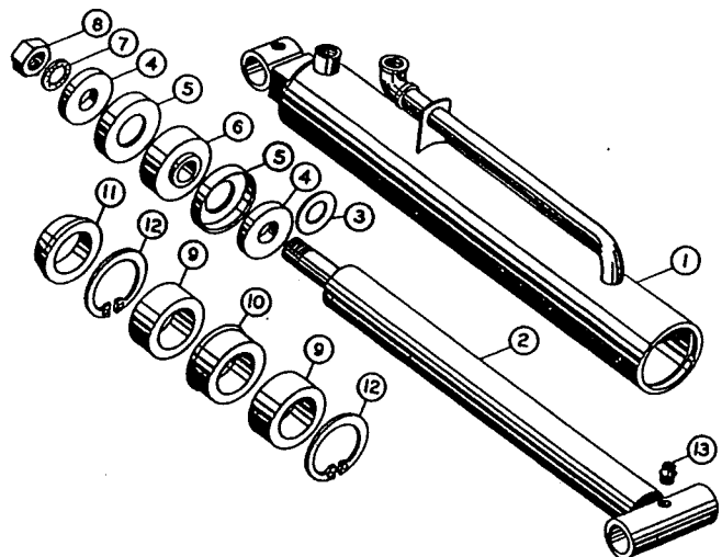
HYDRAULIC CYLINDER - S1 SNAP RING TYPE
