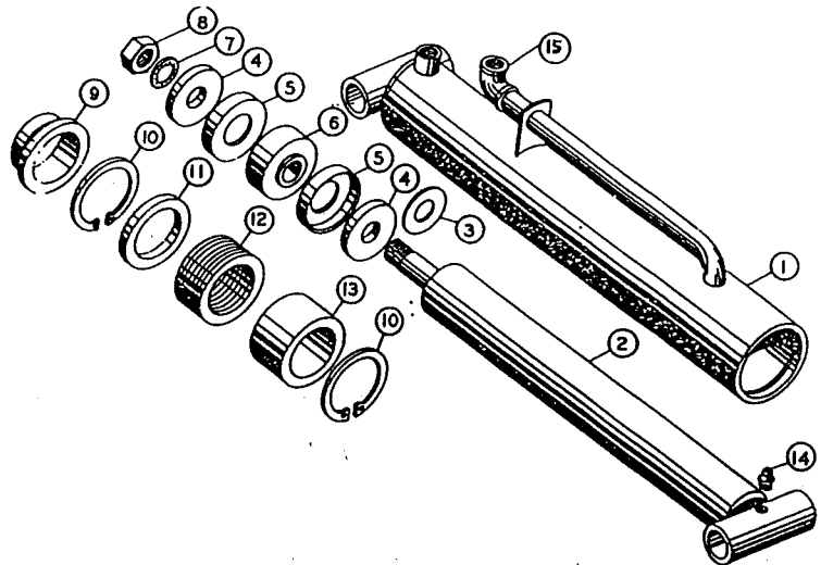
HYDRAULIC CYLINDER SI SNAP RING TYPE
