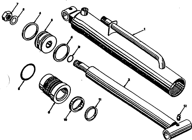
HYDRAULIC CYLINDER - N6 THREADED HEAD TYPE
