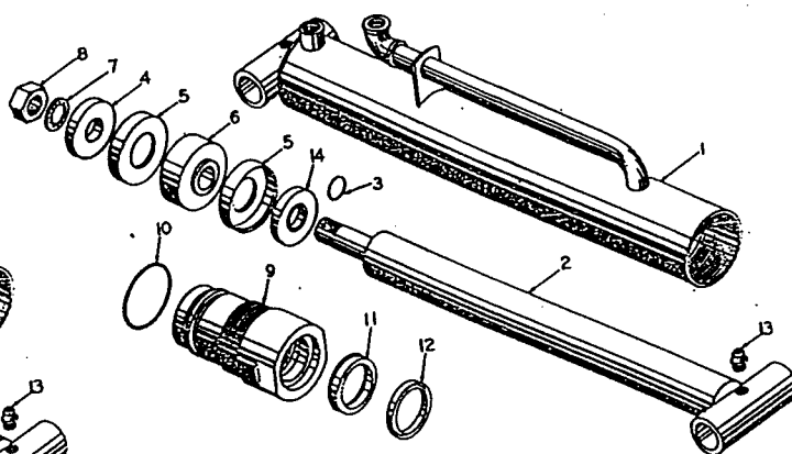
HYDRAULIC SYSTEM - N5 CYLINDER
