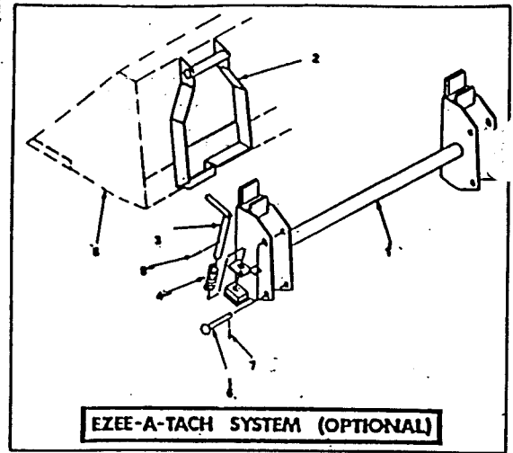
EZEE-A-TACH SYSTEM
