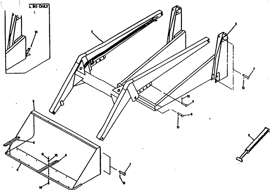
H-FRAME, YOKE AND BUCKET
