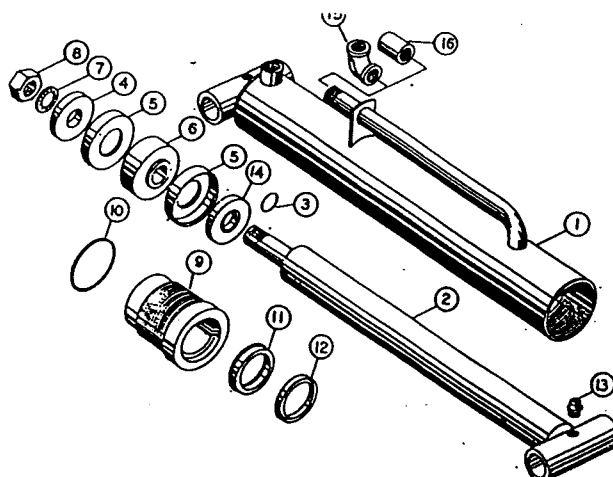
BUCKET AND LIFT CYLINDER - N6 THREADED HEAD TYPE
