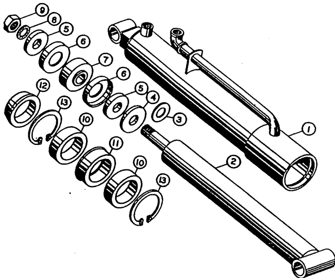
HYDRAULIC CYLINDER - S1-A SNAP RING TYPE
