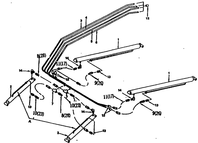
HYDRAULIC SYSTEM (for Models with Serial No. 32094 to 32560)
