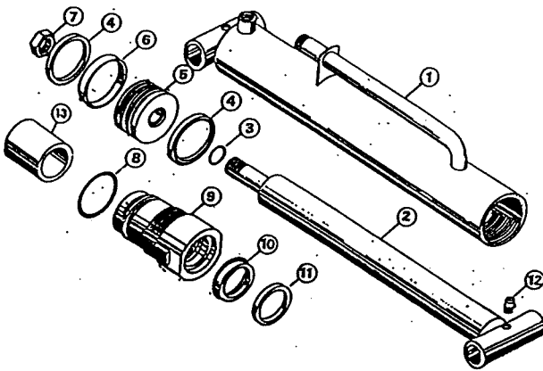
HYDRAULIC CYLINDER DOUBLE "U" CUP PISTON (for Models with Serial no.33735 and up)
