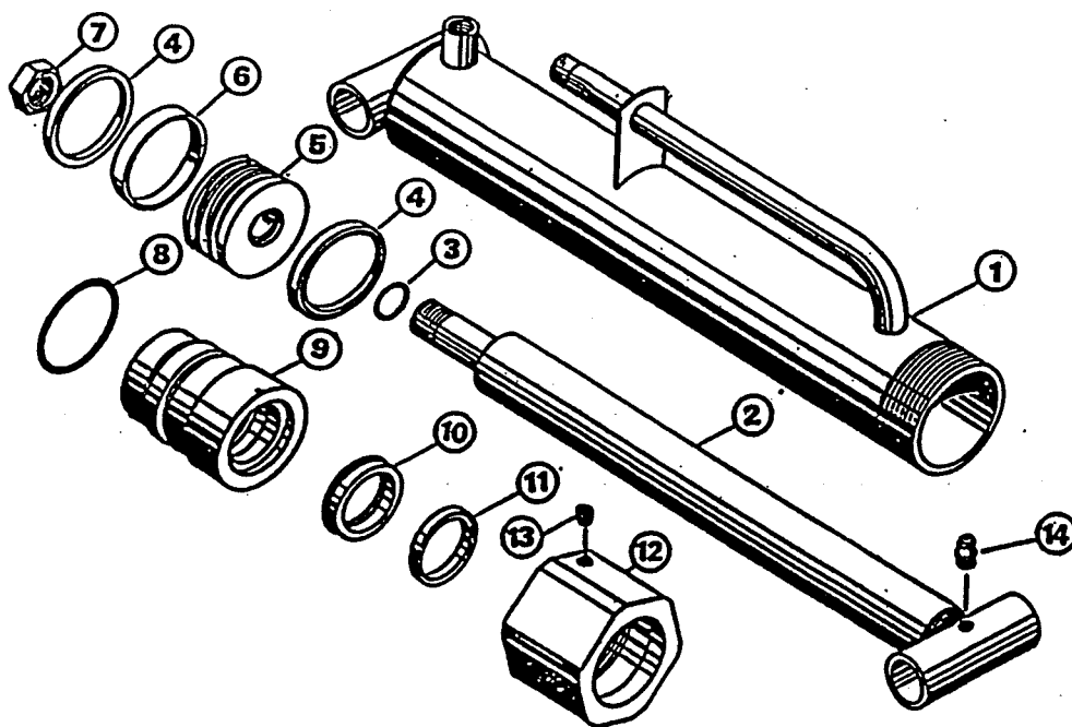
HYDRAULIC CYLINDER (for Model shipped 1992 and later, in Canada) (for Model shipped 1991 and later, in U.S.A.)
