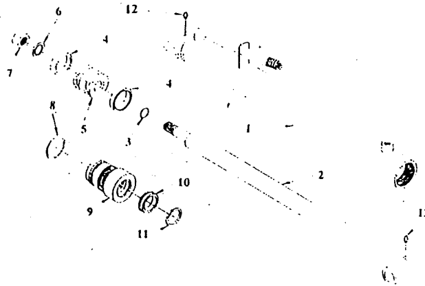
HYDRAULIC CYLINDER ASSEMBLY DOUBLE "U" CUP PISTON - N5 TYPE
