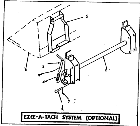
EZEE-A-TACH SYSTEM
