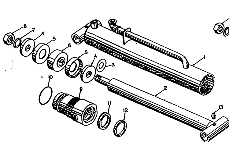
HYDRAULIC SYSTEM - N5 CYLINDER
