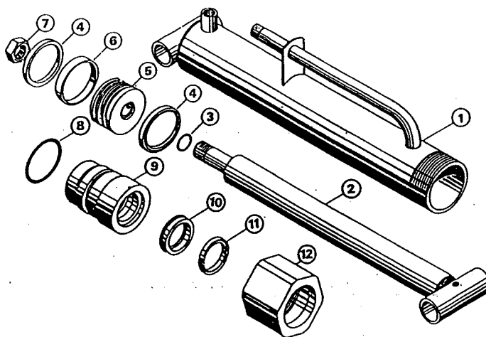
HYDRAULIC CYLINDER - N3 TYPE DOUBLE "U" CUP PISTON
