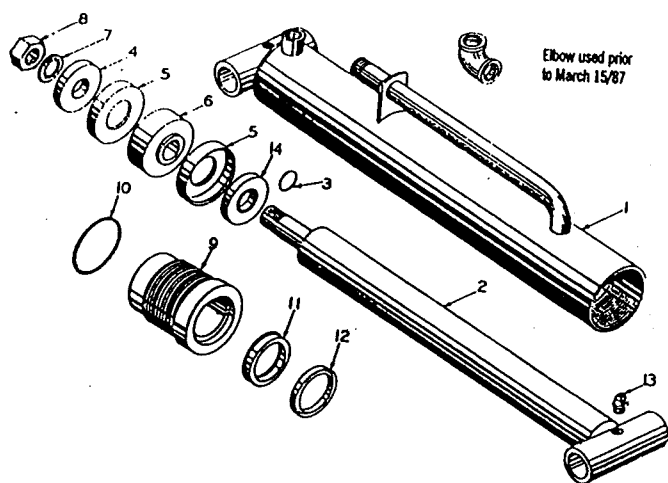
HYDRAULIC CYLINDER - N6 TYPE
