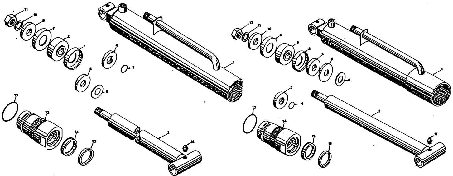
HYDRAULIC CYLINDER - N5 THREADED HEAD TYPE
