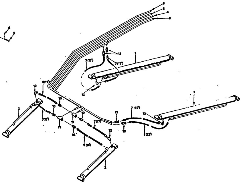
HYDRAULIC SYSTEM
