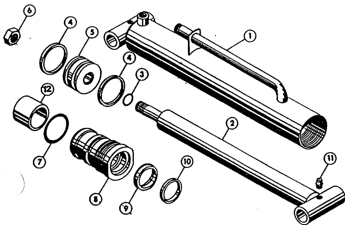
BUCKET CYLINDER N4 THREADED HEAD TYPE DOUBLE "U" CUP PISTON - Less Wear Ring
