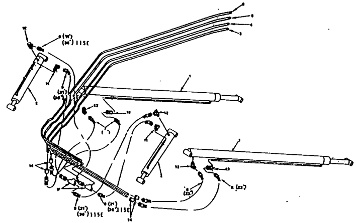
HYDRAULIC SYSTEM (for Model with Serial No. prior to 31583)
