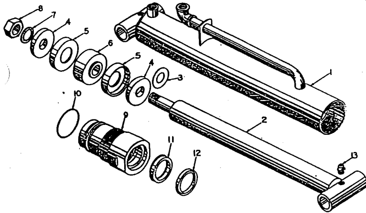
HYDRAULIC SYSTEM - N5 CYLINDER
