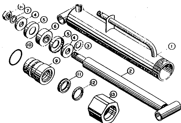
HYDRAULIC CYLINDER - N3 TYPE CYLINDER
