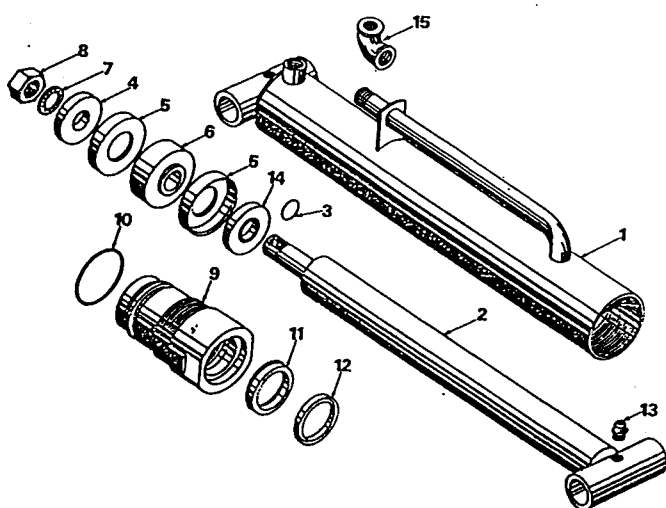
BUCKET CYLINDER - N5 THREADED HEAD TYPE
