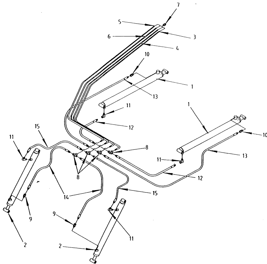
MODEL 2100-2130 HYDRAULIC SYSTEM (FOR MODELS WITH SERIAL NO. 45146 & UP)
