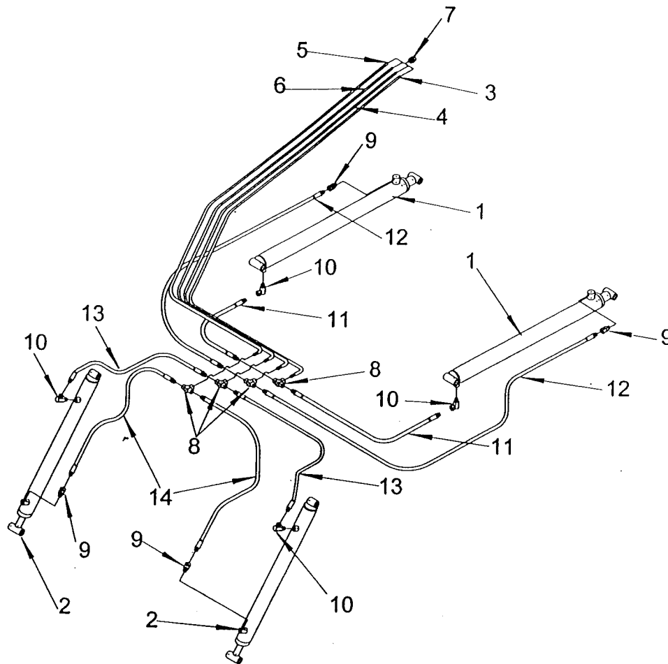
MODEL 2105-2135 HYDRAULIC SYSTEM (FOR SERIAL NOS. 47587 AND UP)
