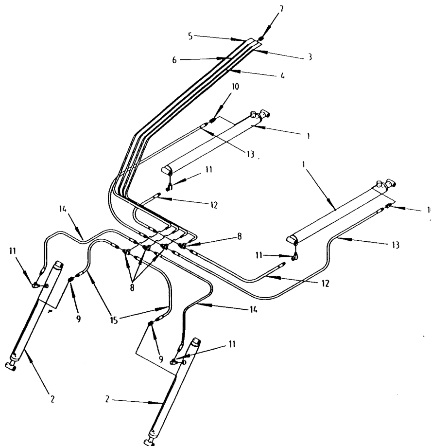
MODEL 2100-2130 HYDRAULIC SYSTEM (FOR MODELS PRIOR TO SERIAL NO. 45146)
