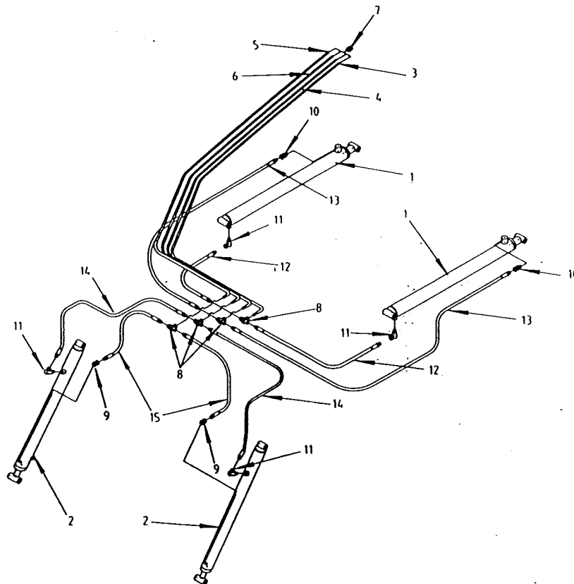
MODEL 2105-2135 HYDRAULIC SYSTEM (For Model 2135 Prior to S/N 47587)
